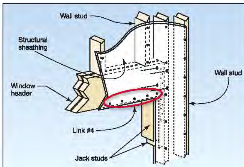
Figure 9-13. Connection of wall sheathing to window header (Link #4)
