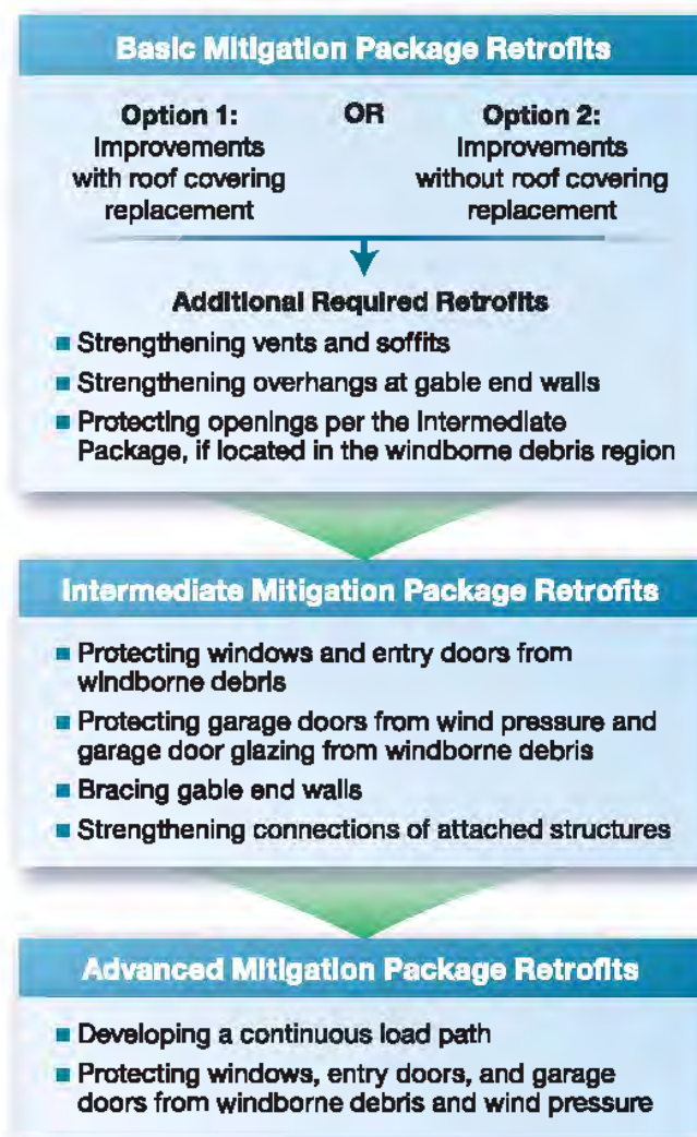
Figure 15-15. Wind Retrofit Mitigation Packages
